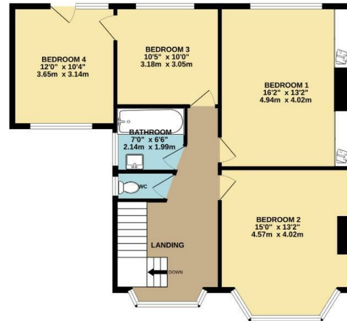
1ST FLOOR 828 sq.ft. (76.9 sq.m.) approx.
